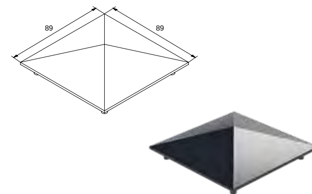
Code: 4485 ABDECKUNG PFOSTEN 80x80 CLS-100
